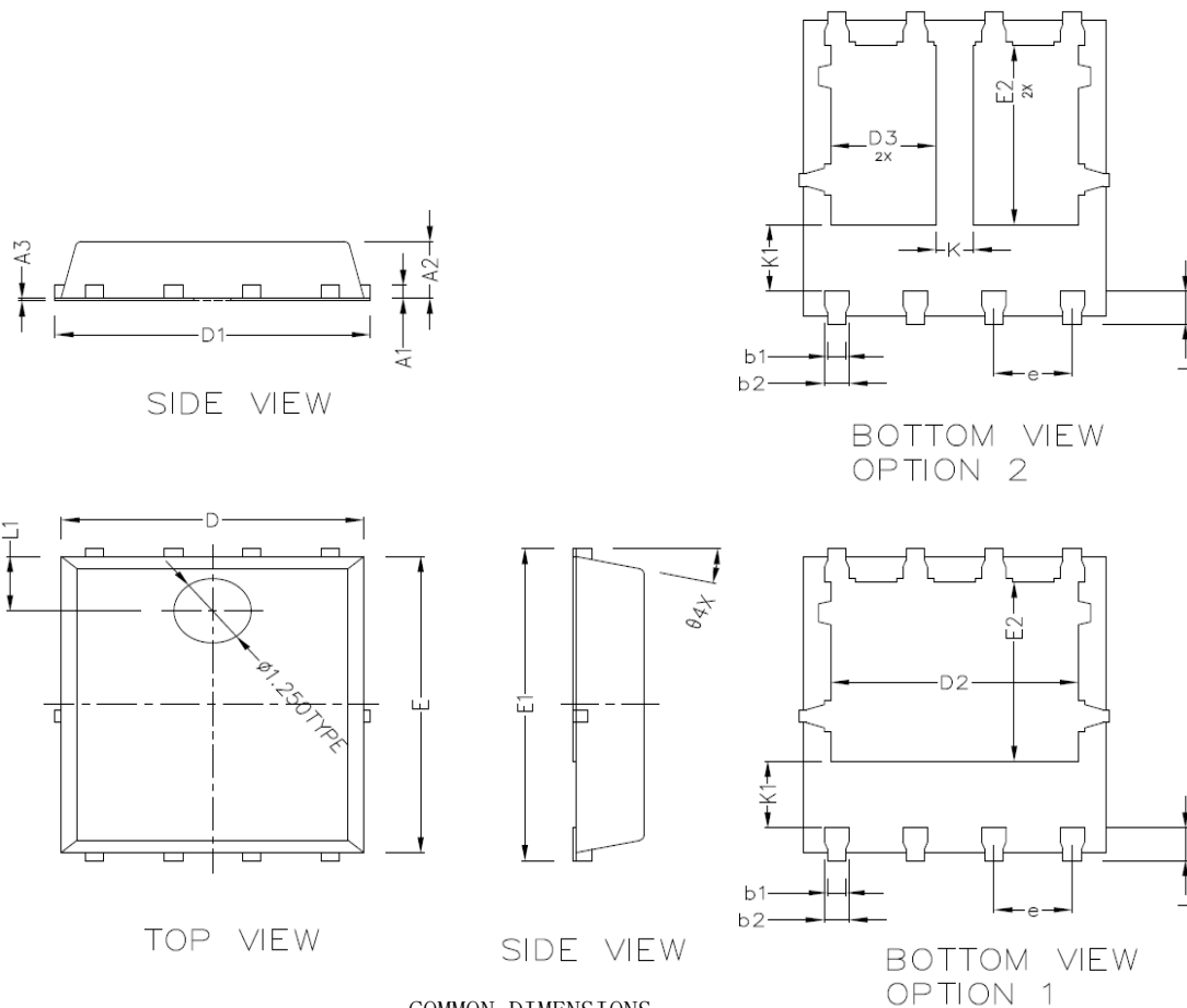
COMMON DIMENSIONS (UNITS OF MEASURE IS mm)
